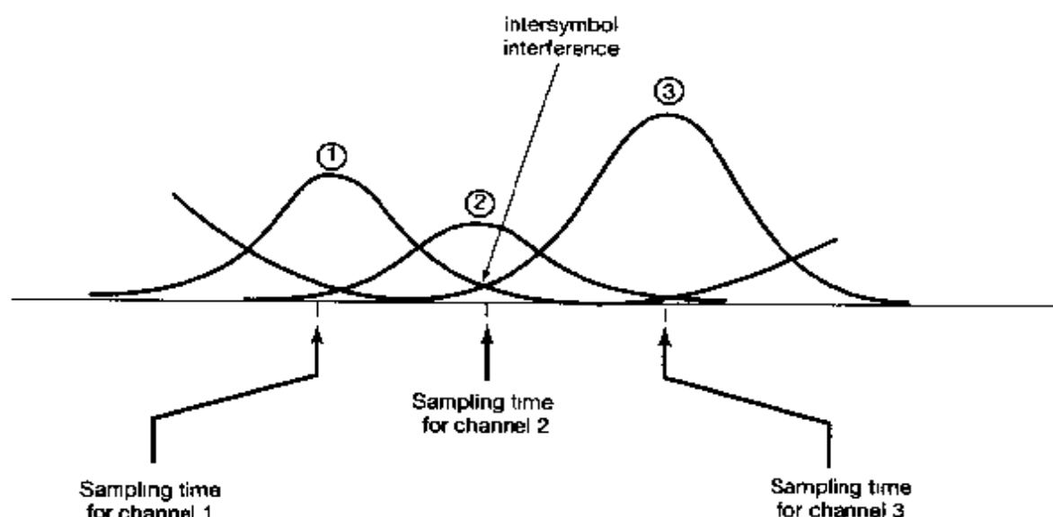
Figure 8.28 Intersymbol Interference.
