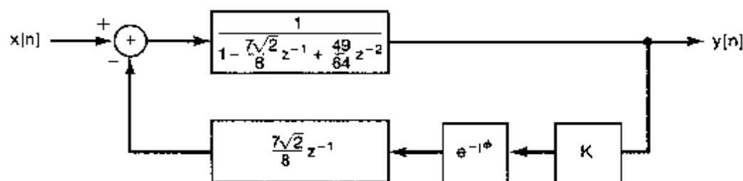
Figure 11.33 Discrete-time feedback system of Example 11.13.
