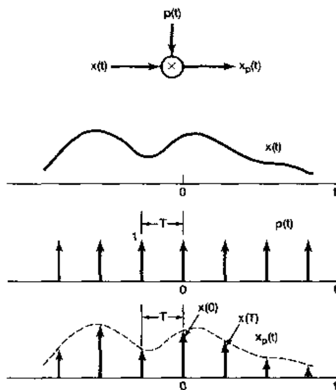
Figure 7.2 Impulse-train sampling.
