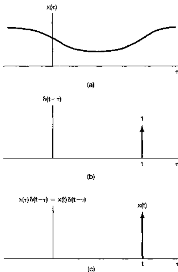
Figure 2.14 (a) Arbitrary signal x(\tau) ; (b) impulse \delta(t - \tau) as a function of \tau with t fixed; (c) product of these two signals.
