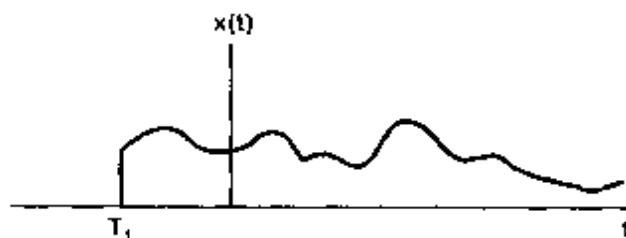
Figure 9.6 Right-sided signal.
