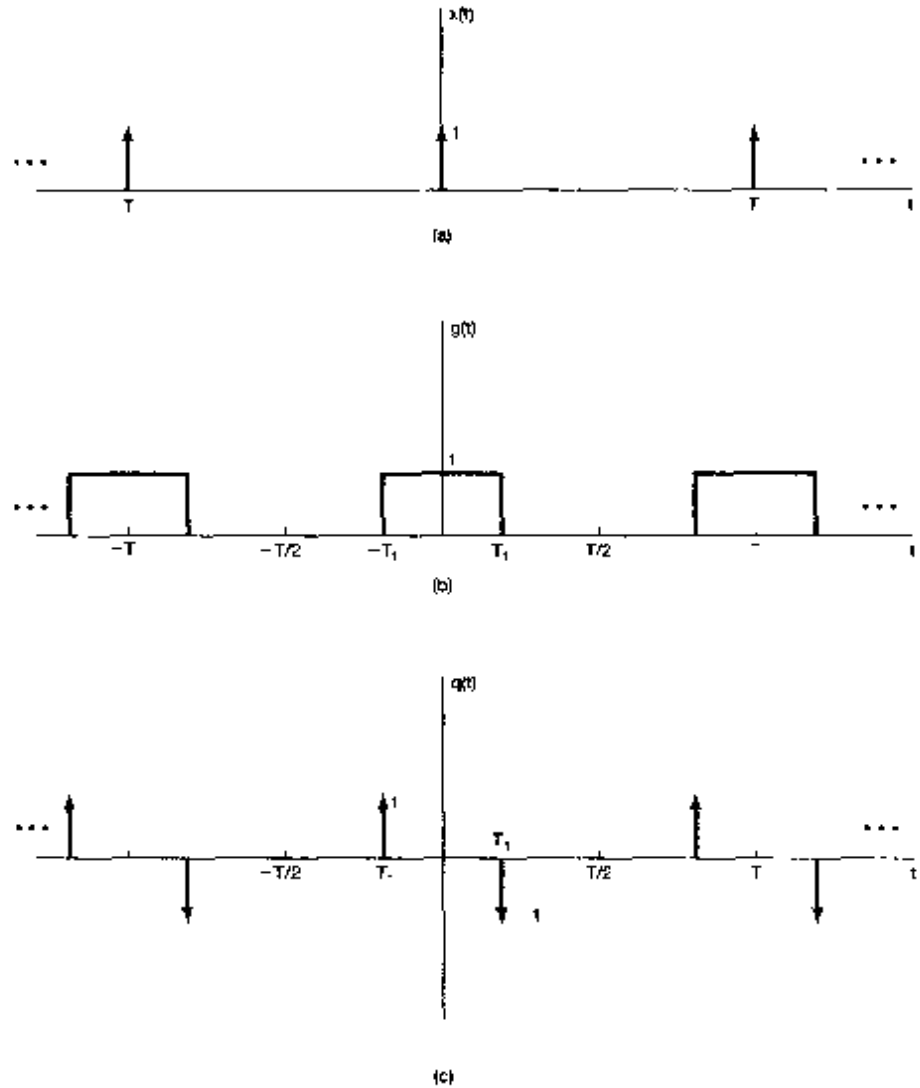
Figure 3.12 (a) Periodic train of impulses, (b) periodic square wave; (c) derivative of the periodic square wave in (b).
