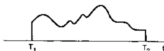
Figure 9.4 Finite-duration signal.
