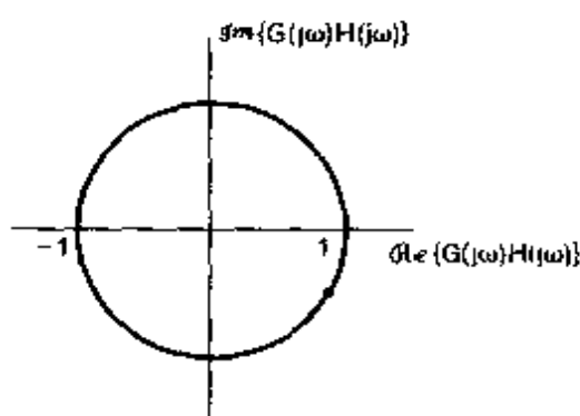
Figure 11.23 Nyquist plot for Example 11.7.
