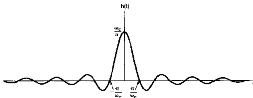
Figure 4.21 Impulse response of an ideal lowpass filter.
