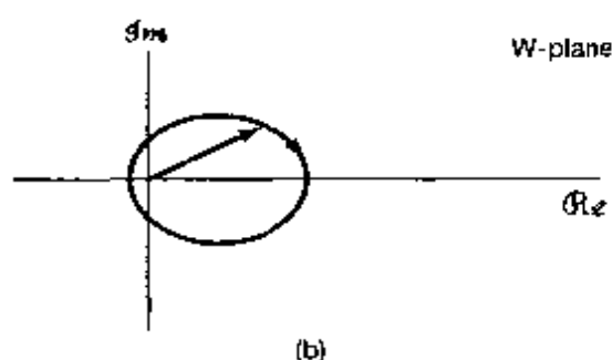
Figure 11.17 Basic encirclement property. The closed curve in (b) represents a plot of the values of W(p) for values of p along the curve C in (a). Here, the arrow on the curve C in (a) indicates the direction in which C is traversed, and the arrow in (b) indicates the corresponding direction along the contour of values of W(p) .
